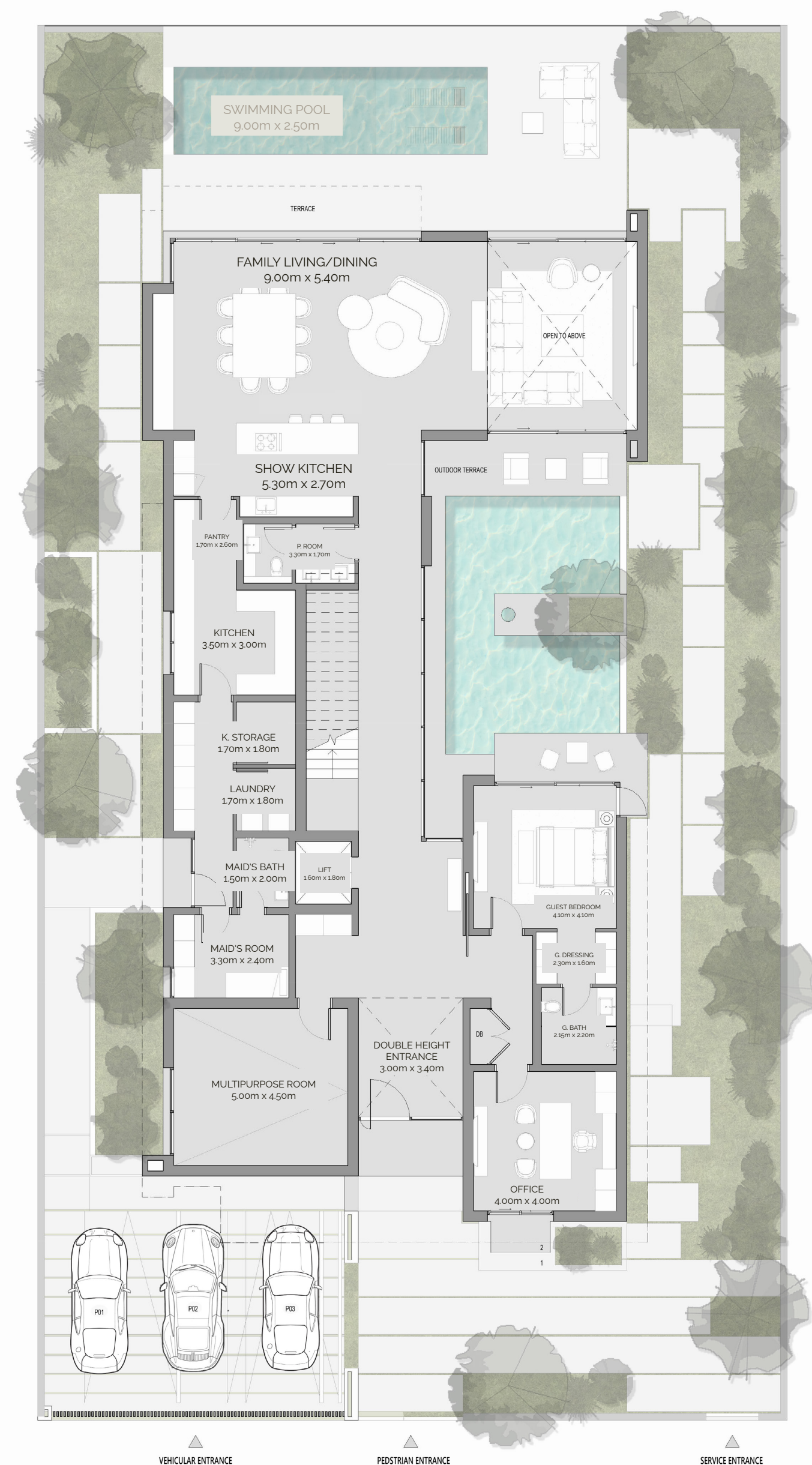
GROUND FLOOR
