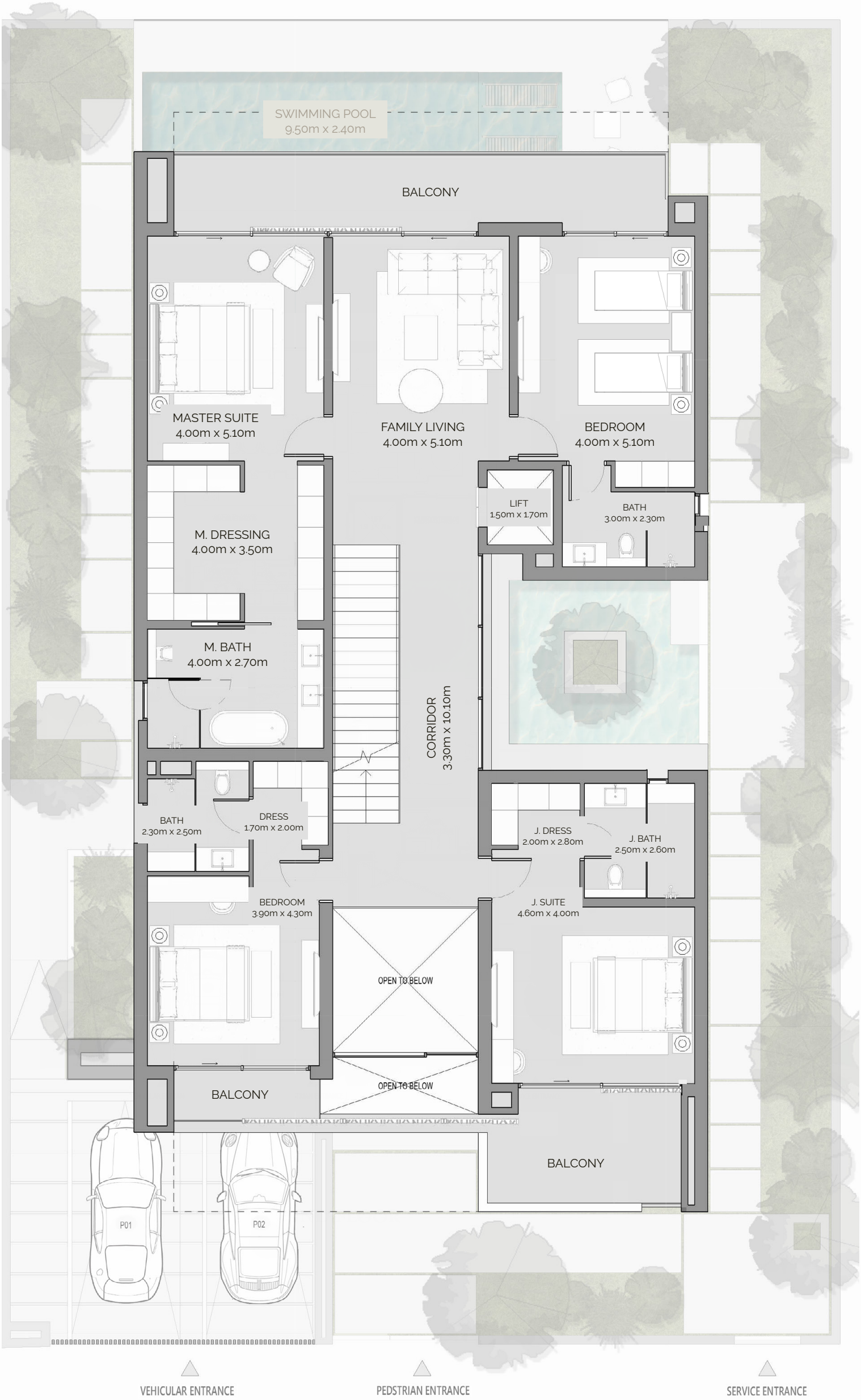
FIRST FLOOR
