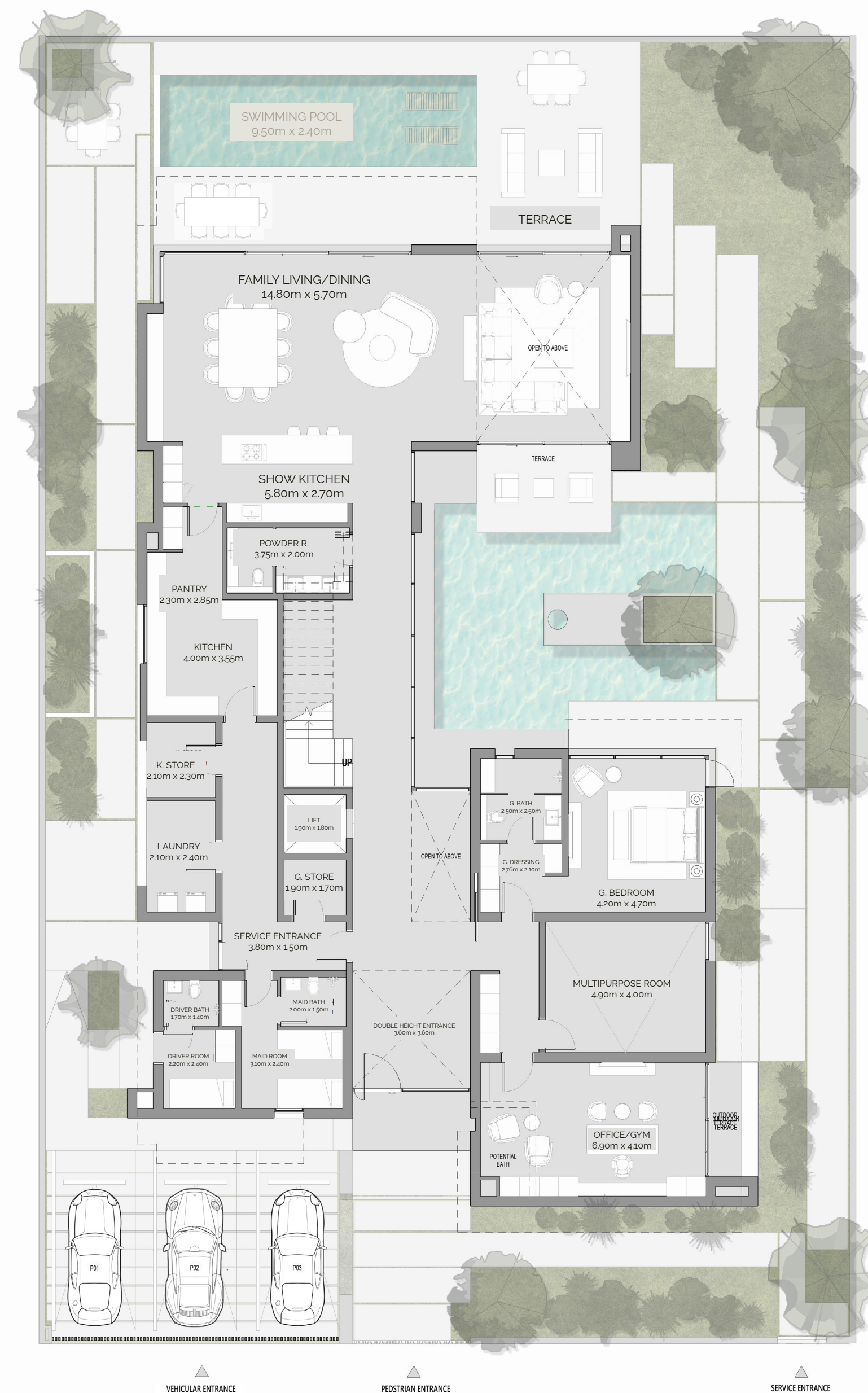
GROUND FLOOR
