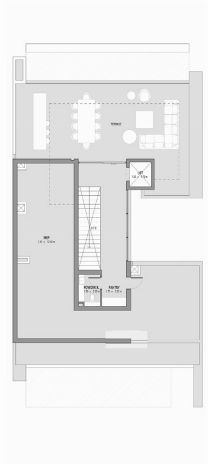
Roof Floor
